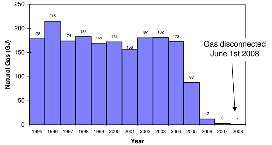
Annual Natural Gas Consumption at the Mills Residence 1995 - 2008
