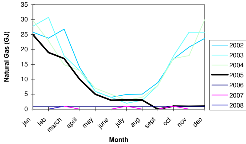
Monthly Natural Gas Consumption at the Mills Residence 2001 - 2008
